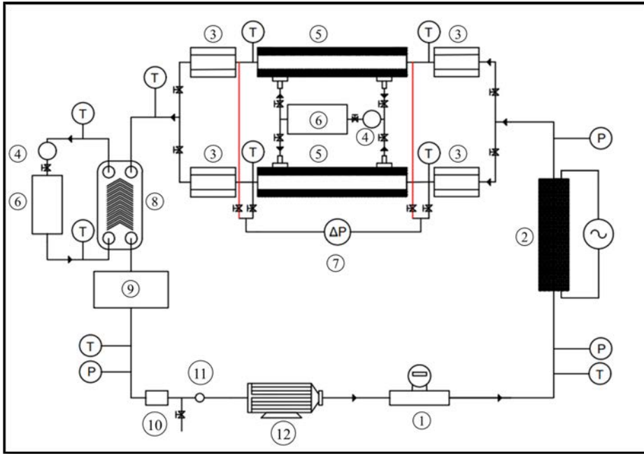
管內冷凝測試設備 Condensation test facility of internal flow
